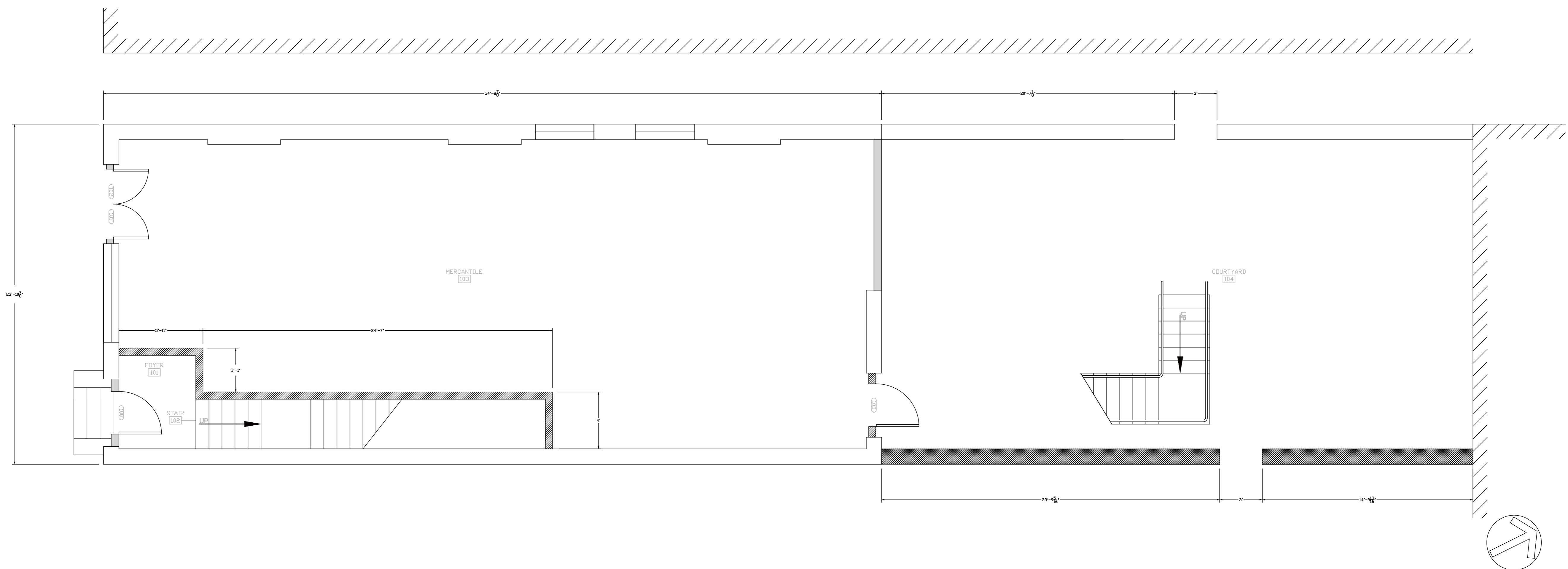
1 FIRST FLOOR DIMENSION PLAN A1.1.1 SCALE 1/4" = 1'
